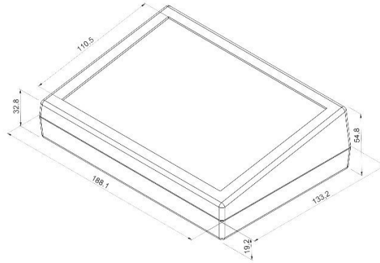
Figure 2: AT550 technical drawings
